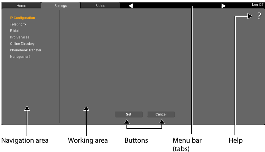
Image 2 Example of the structure of a Web configurator page
